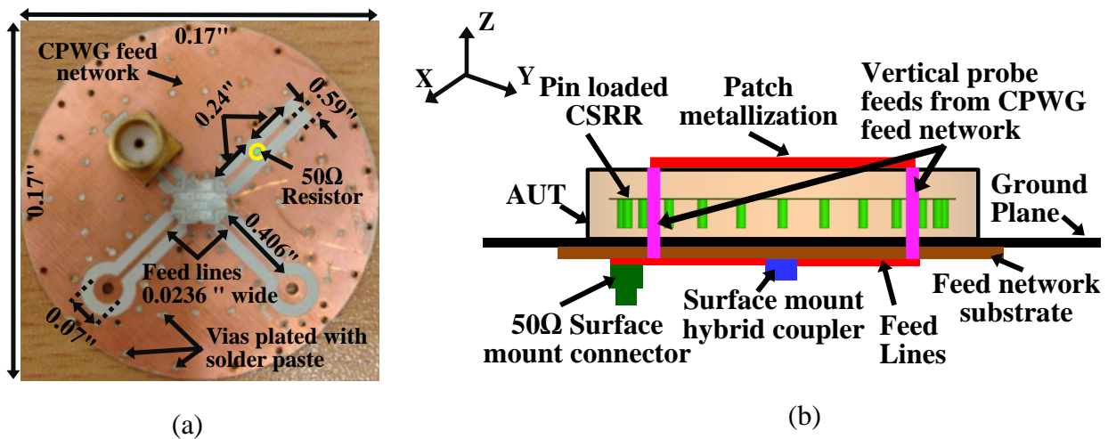
Figure 4.6: Fabricated antenna feed structure. (a) Layout with dimensions; (b) Illustration of the feed mounting over the 24'' \times 24'' \times 0.025'' brass ground plane.
